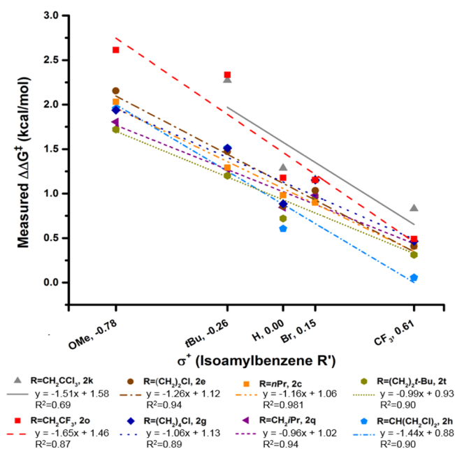
Figure 5. Plot of measured \Delta\Delta G^\ddagger versus Hammett \sigma^+ for the DoE set of sulfamate esters evaluated in the isoamylbenzene substrate series R' = OMe ( 1a ), t\text{-Bu} ( 1c ), H ( 1 ), Br ( 1d ), CF_3 ( 1b ). \Delta\Delta G^\ddagger = -RT \ln(\text{tertiary/benzylic}) , where T is 23 °C. Omitted from this plot are data points corresponding to R = CH_2CCl_3 , R' = OMe (benzylic-to-tertiary ratio >100:1) and R = CH(CH_2Cl)_2 , R' = Br (no measurable products observed).
