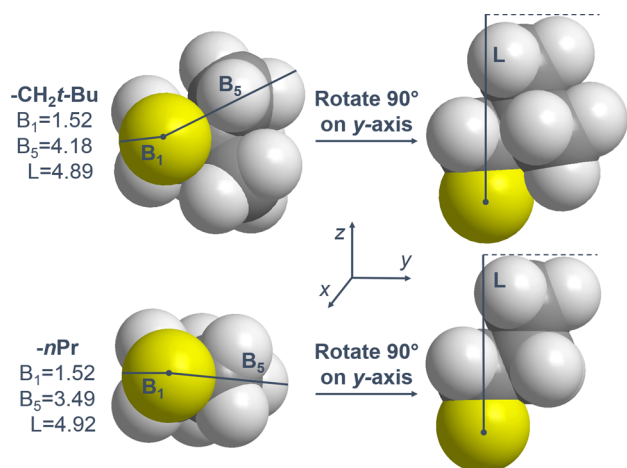
Figure 3. Schematics of the Sterimol parameter system, describing the subparameters B_1 (minimum radius), B_5 (maximum radius), and L (length). Comparisons of nPr and CH_2t\text{-Bu} demonstrate a deficiency in the Sterimol parameters, where sterically distinct groups are similarly described.
